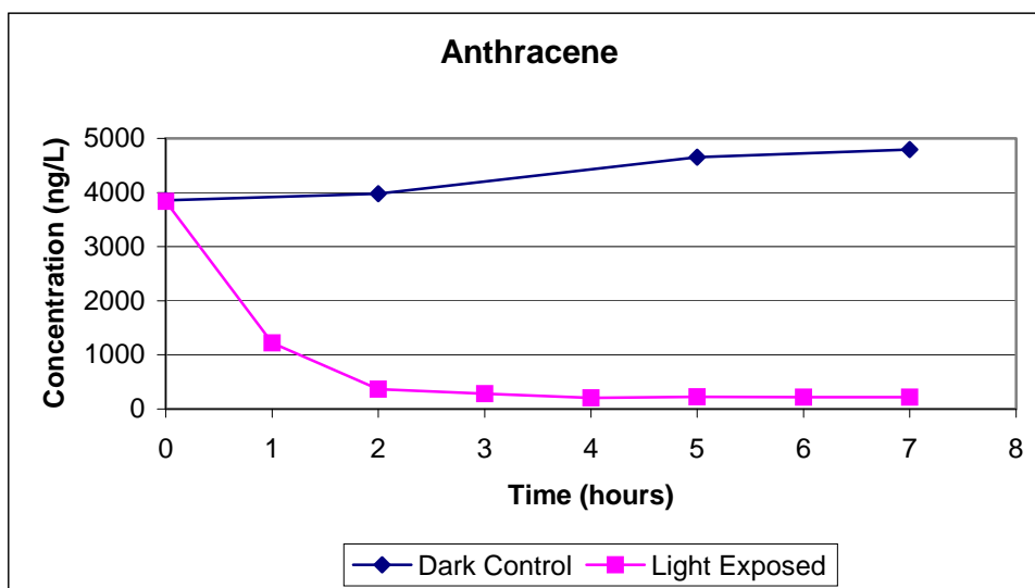
Figure 3.2.3. Photochemical degradation of anthracene in distilled water.
