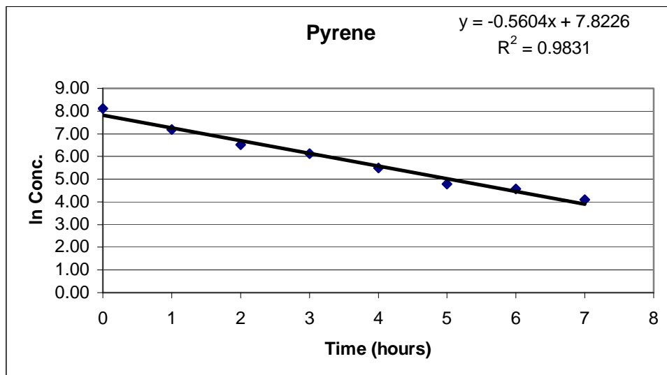
Figure 3.2.4. First order loss of pyrene in water contaminated by a 2-cycle engine.
