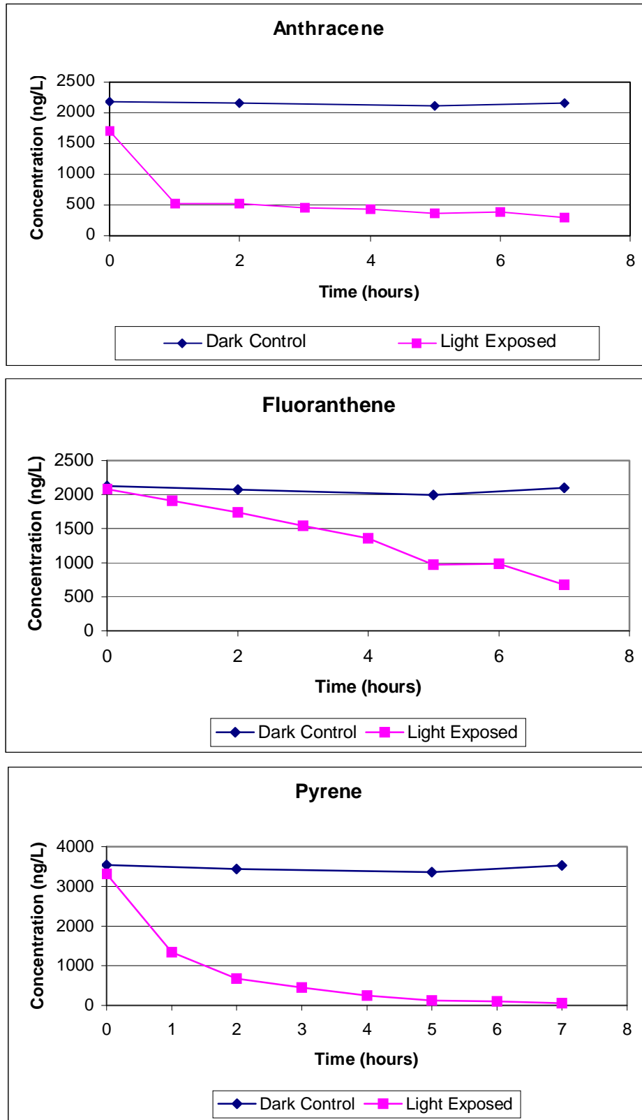
Figure 3.2.2. Photochemical degradation of anthracene, fluoranthene, and pyrene from 9.9 hp 2-stroke engine contaminated water.
